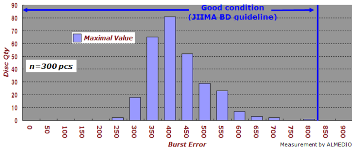
BD-R 50GB Initial Characteristics Burst Error
