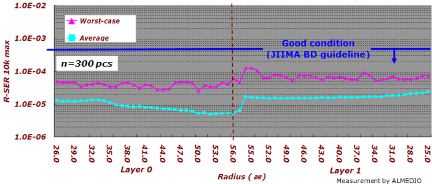
BD-R 50GB Initial Characteristics R-SER
